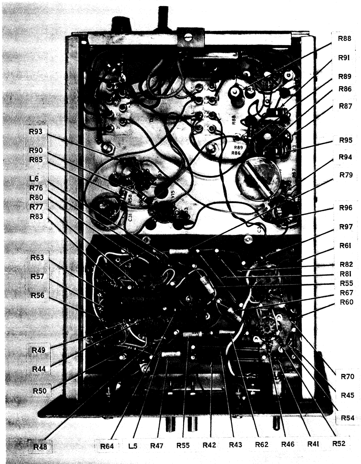
Figure 6-8. Signal Generator SG-299B/U, SG-299D/U, and SG-299E/U, parts location, bottom view, part 1.
