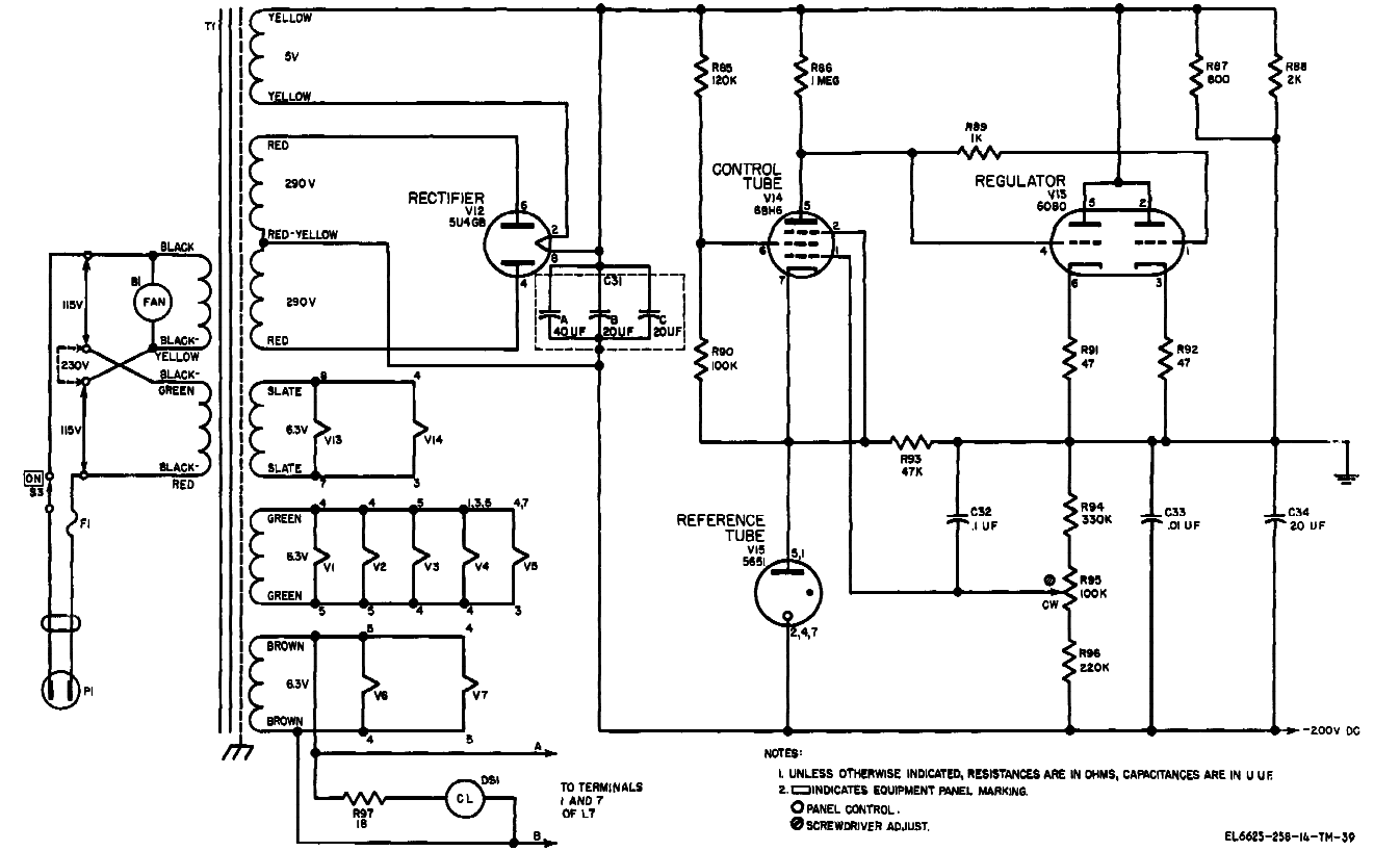
Figure FO-4. Signal Generator (SG-299/U, power supply, schematic daigram.
