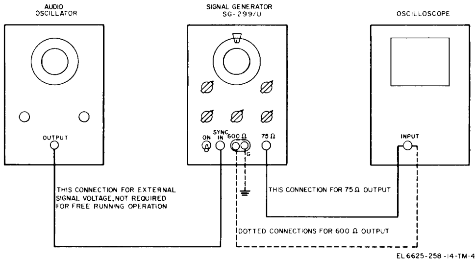
Figure 3-2 Test setup.
