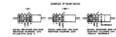
A. COLOR CODE MARKING FOR MILITARY STANDARD RESISTORS. B. COLOR CODE MARKING FOR MILITARY STANDARD INDUCTORS.
