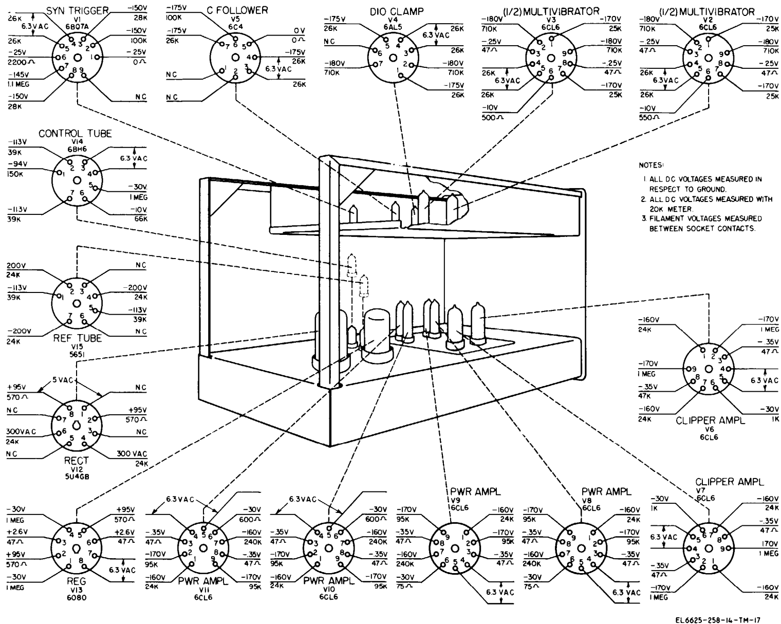
Figure 6-1. Tube socket voltage and resistance diagram (unlettered, B, D, and E models).
